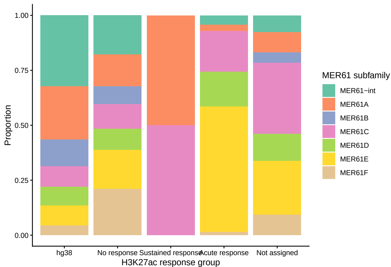
MER61 subfamily composition across H3K27ac sets
